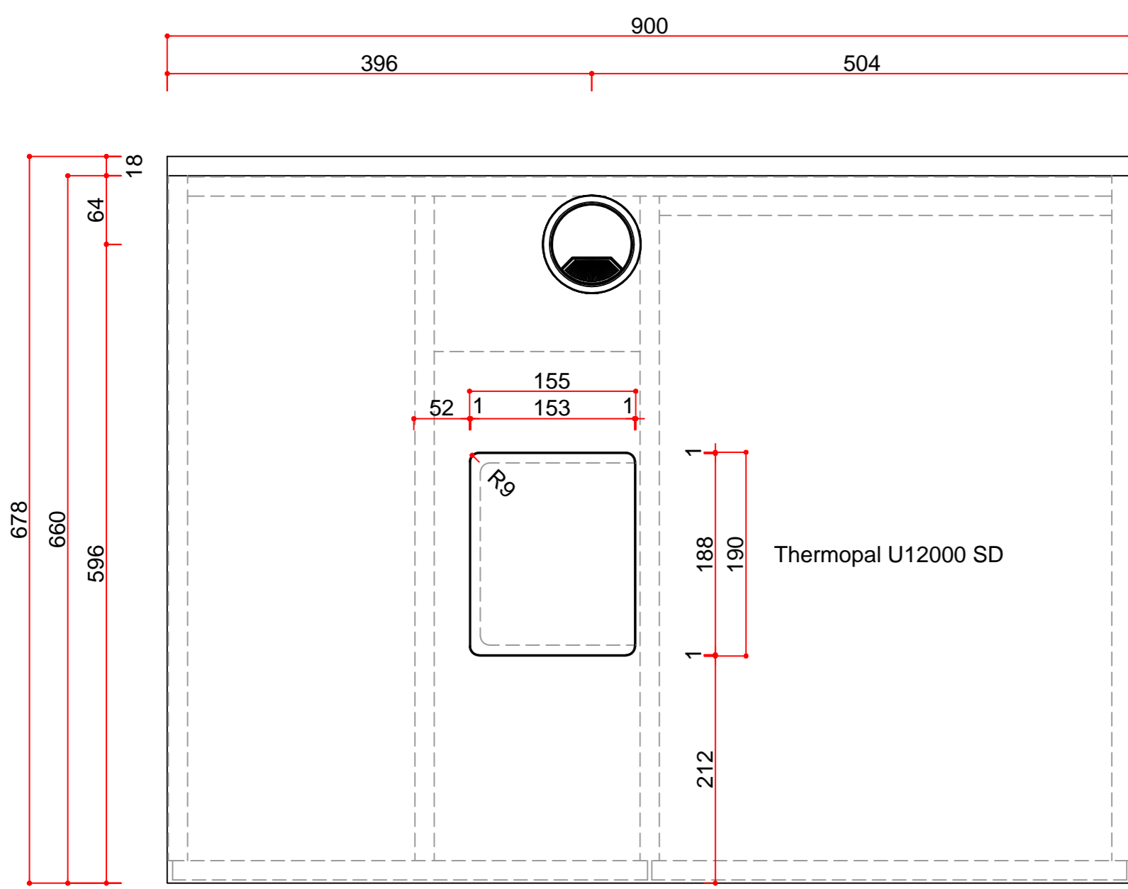
Top view
