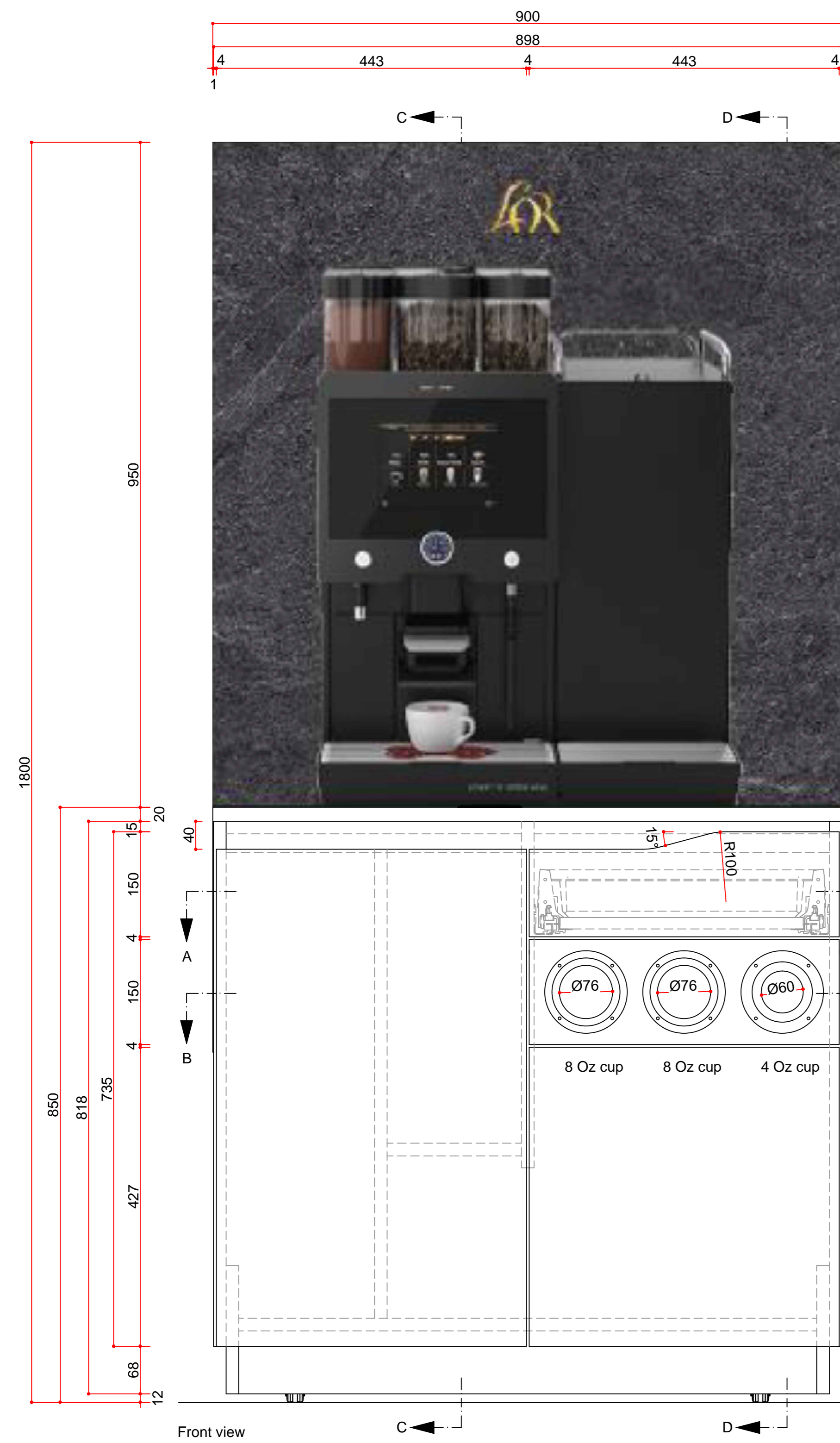
Front view
