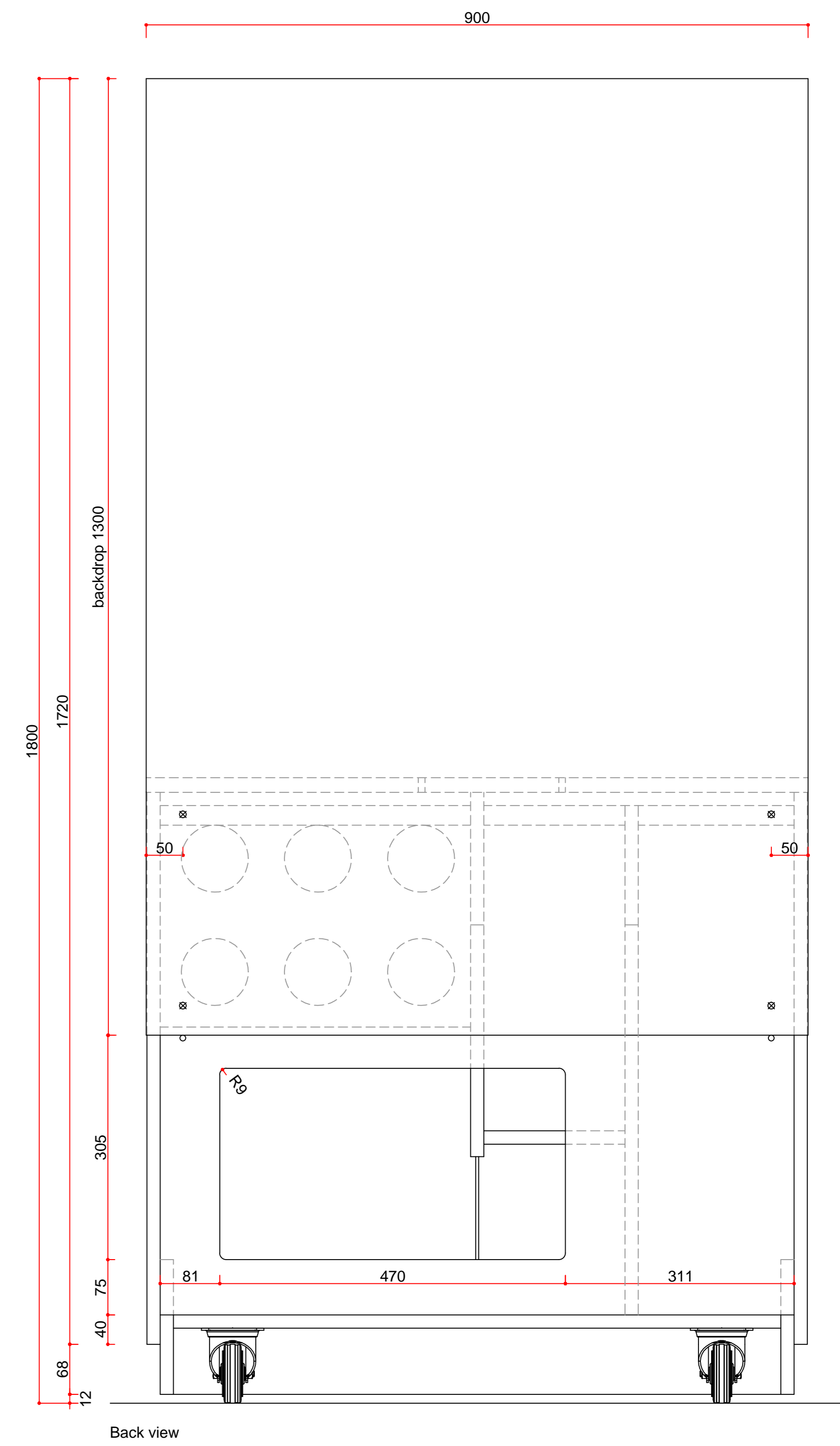
Back view
