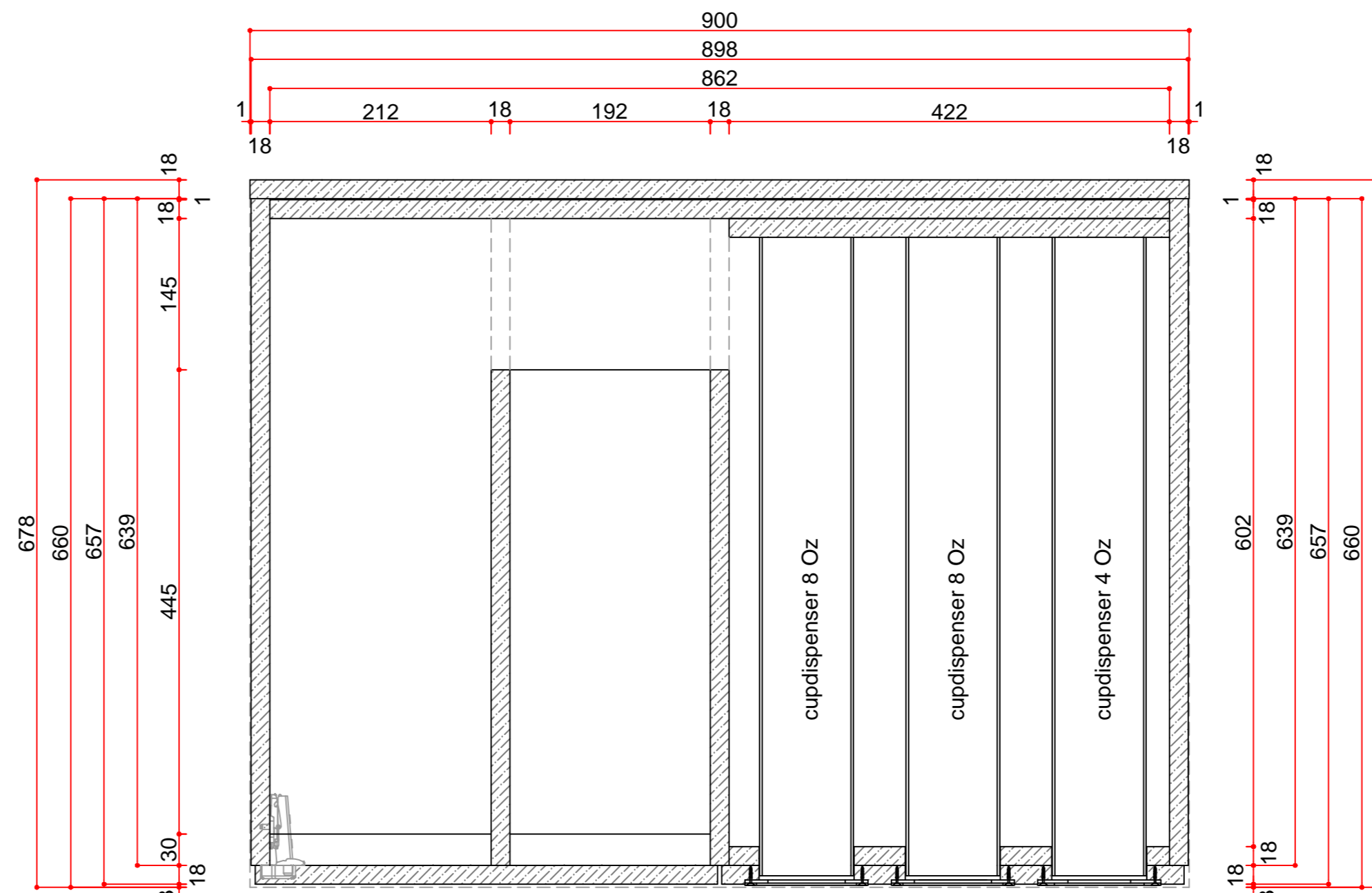
Horizontal section B-B
