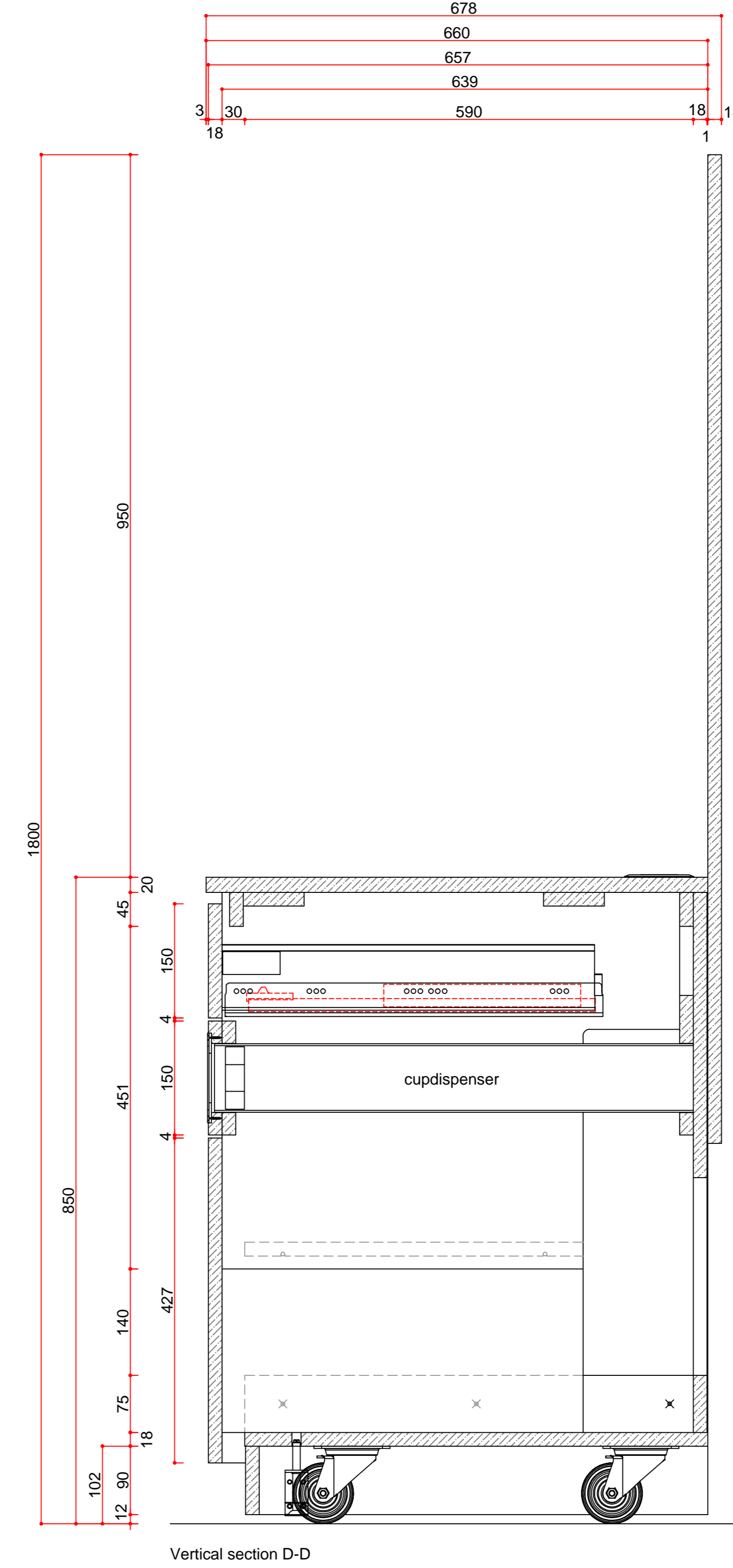
Vertical section D-D
