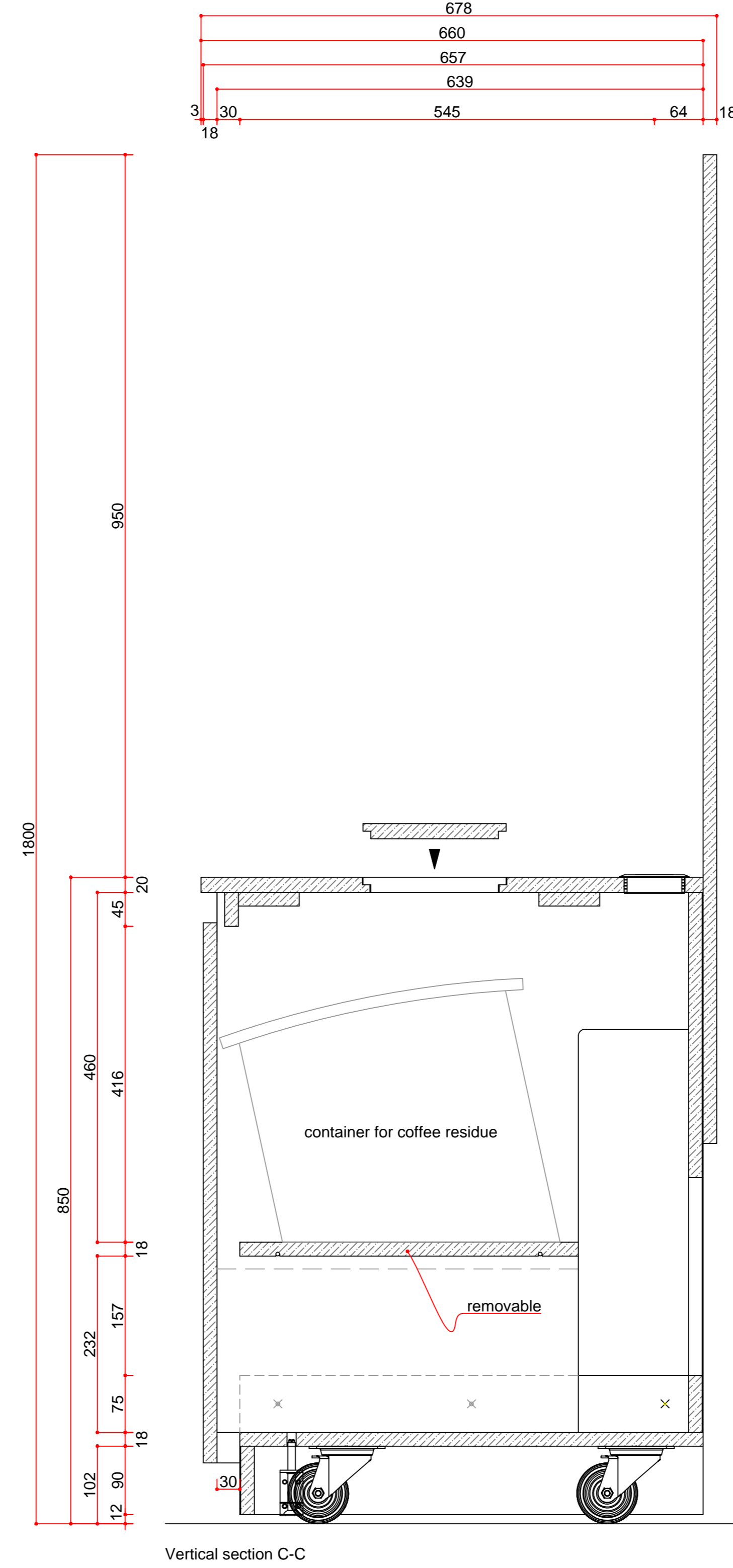
Vertical section C-C
