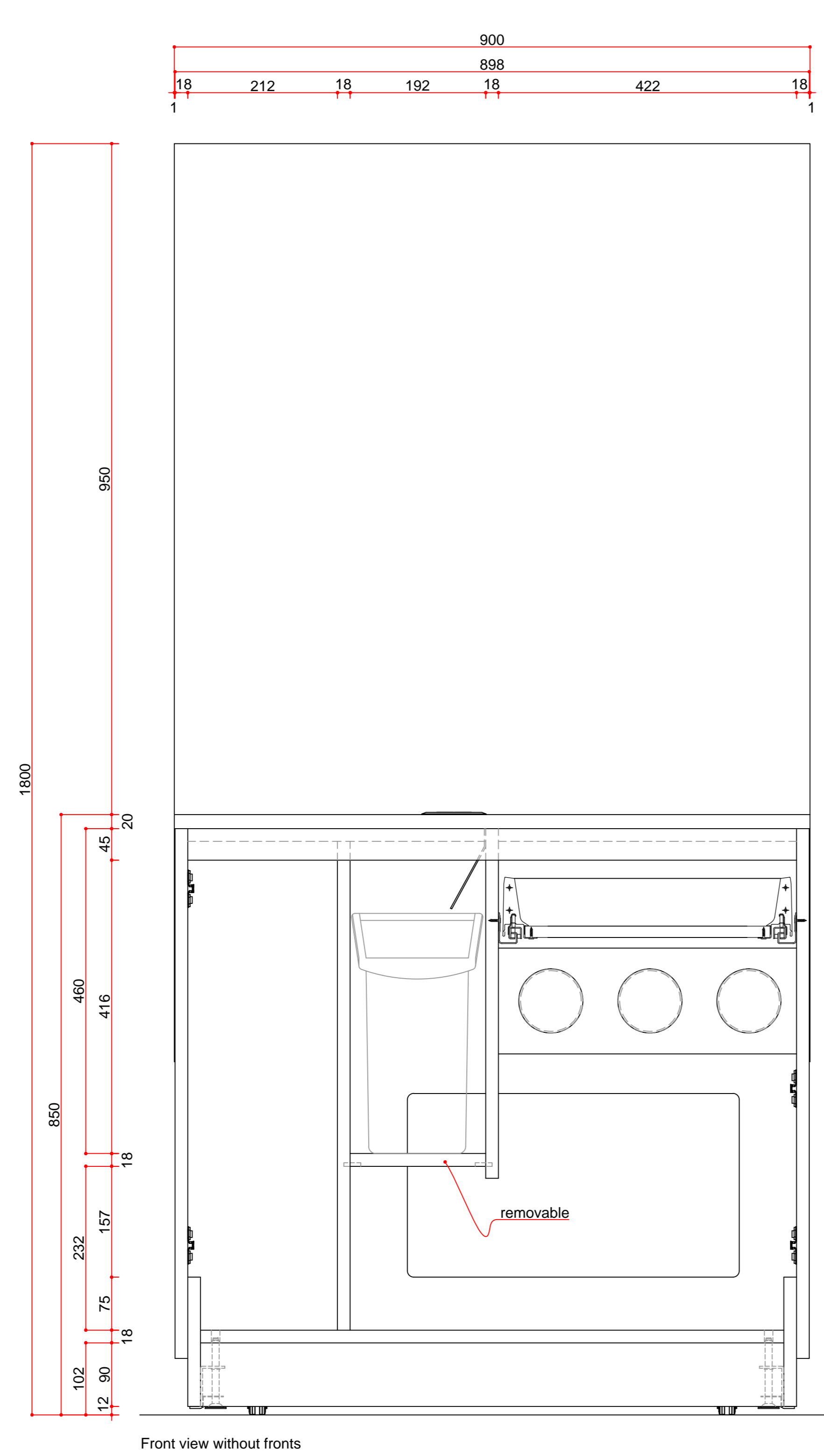
Front view without fronts
