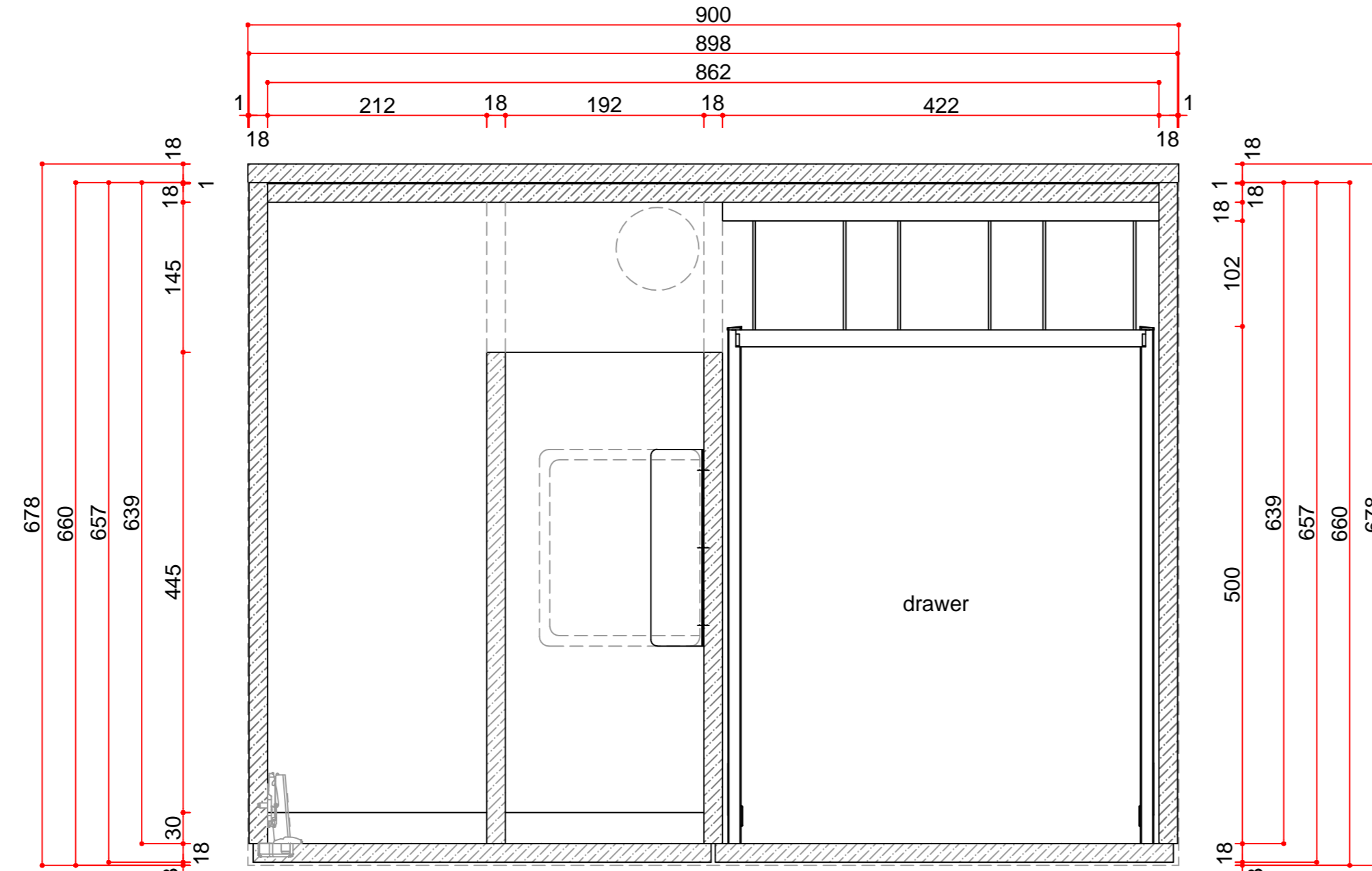
Horizontal section A-A
