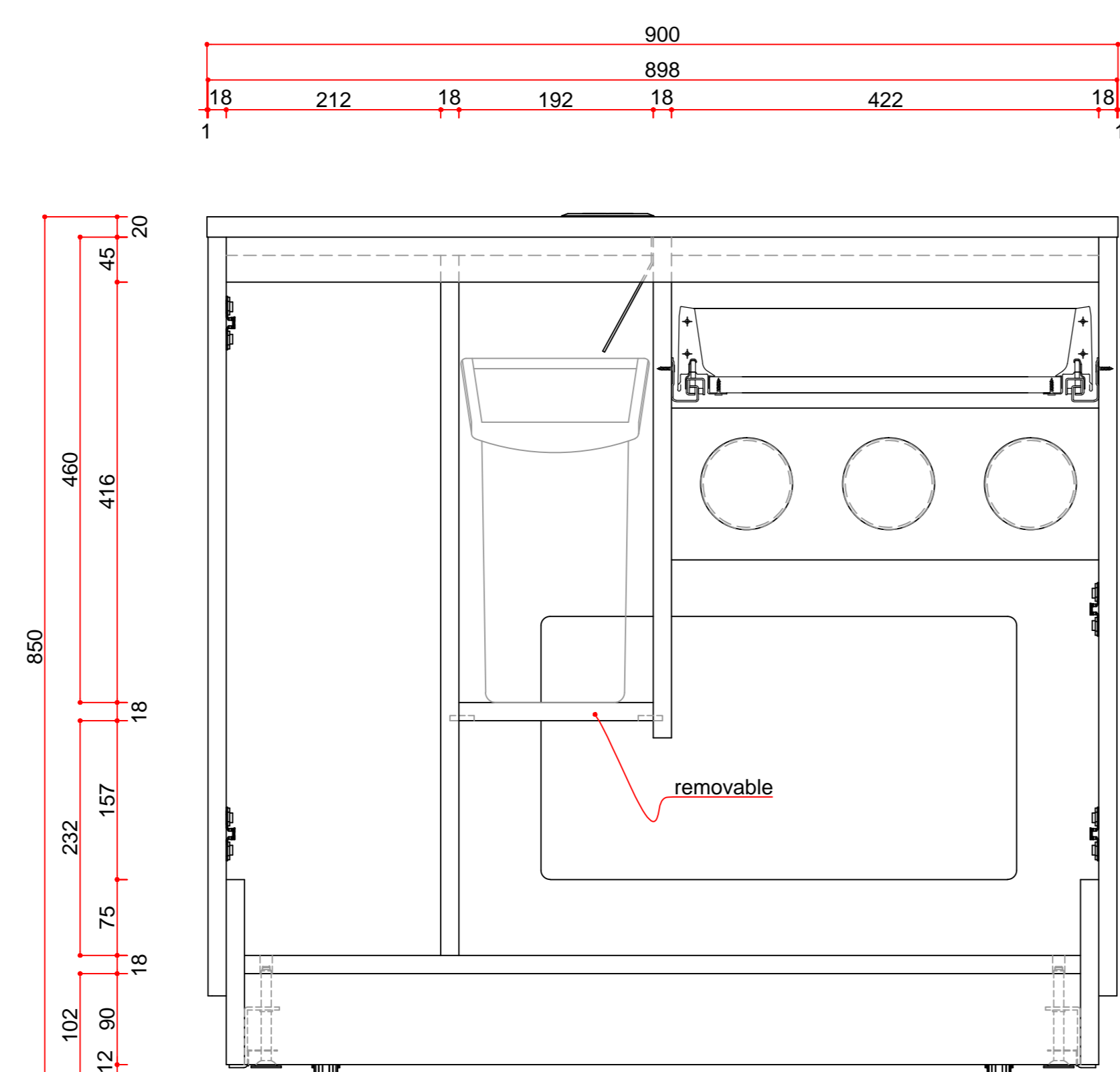
Front view without fronts
