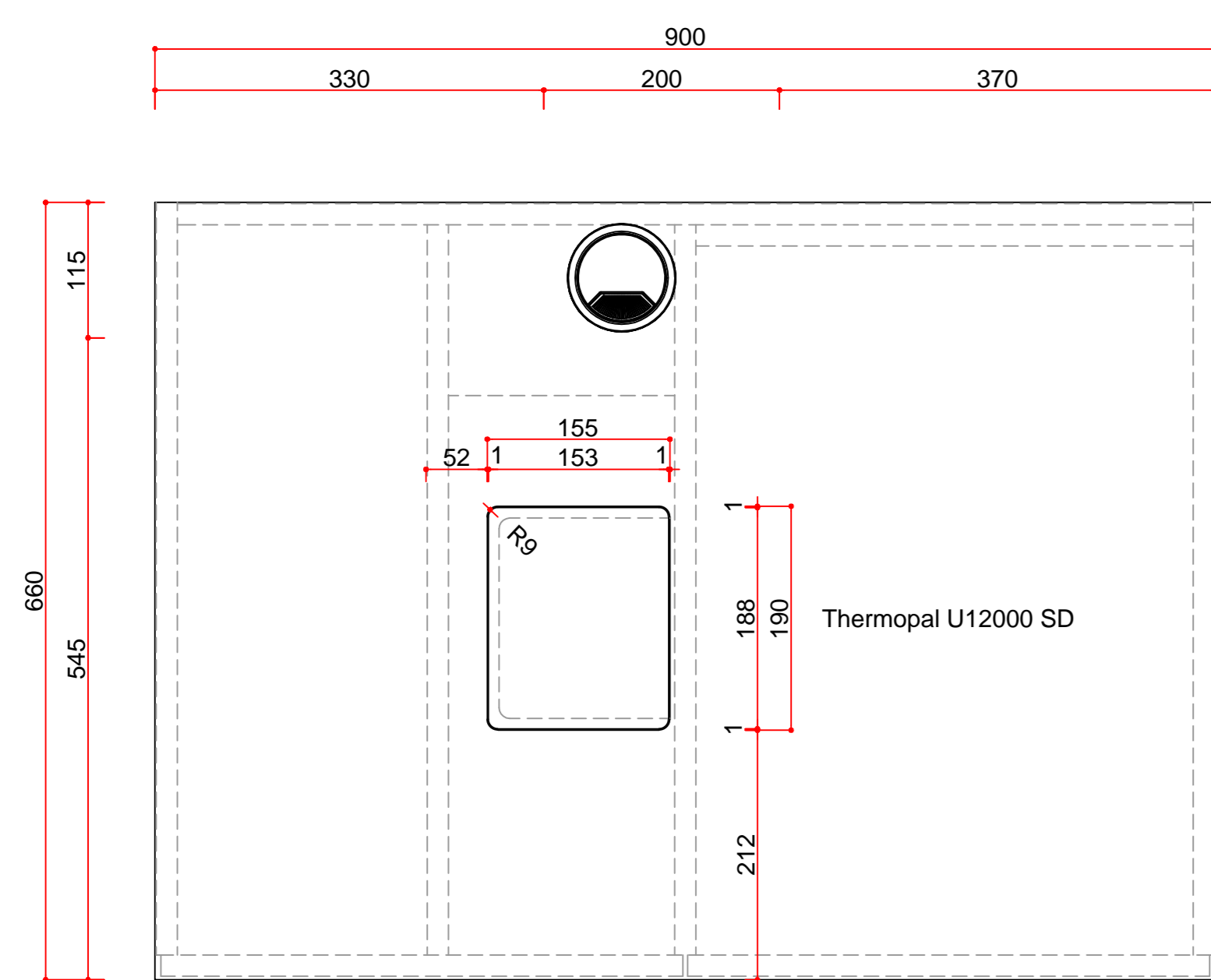
Top view
