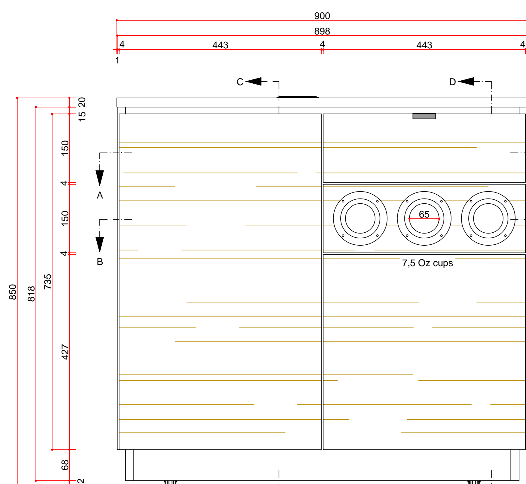
Front view
