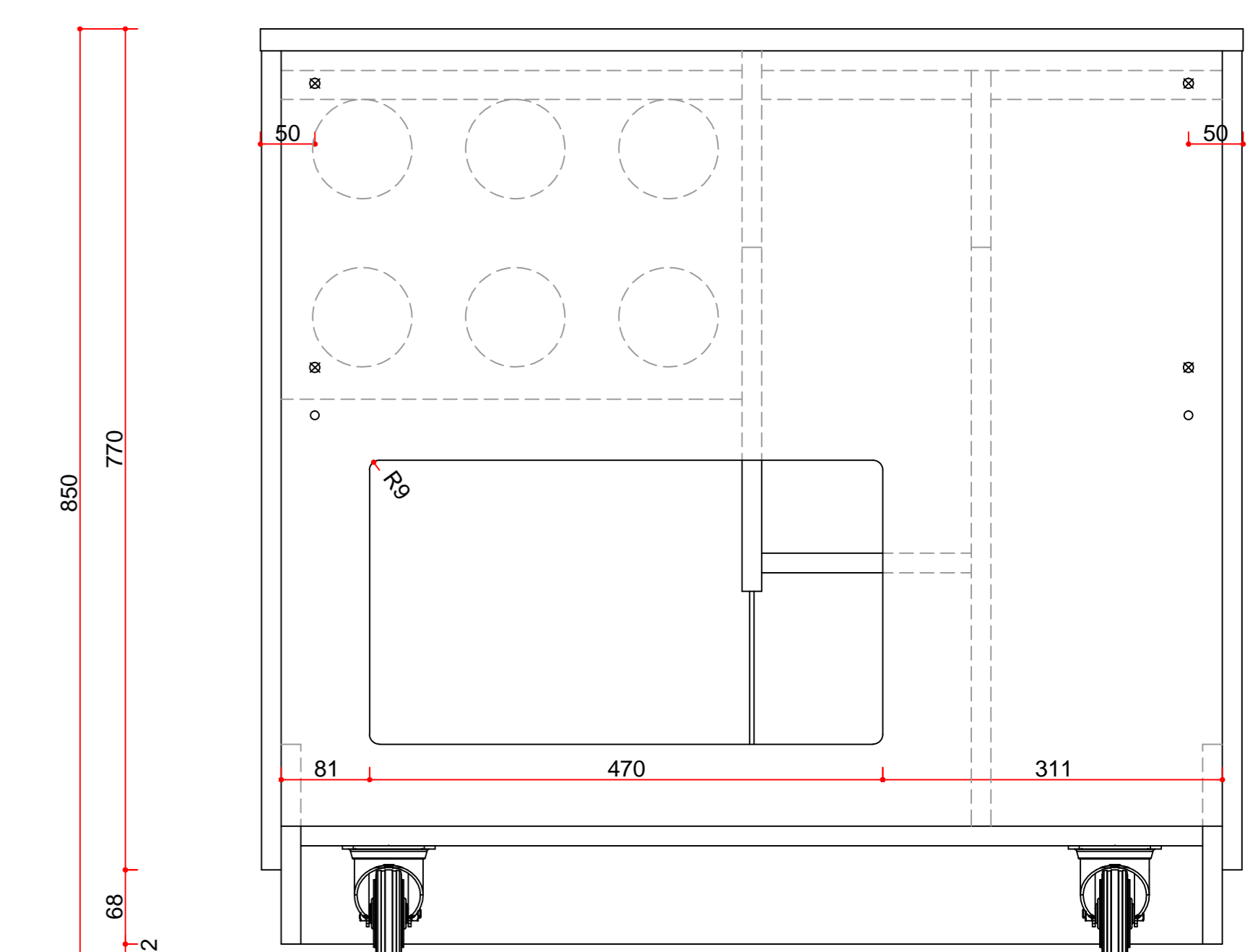
Back view
