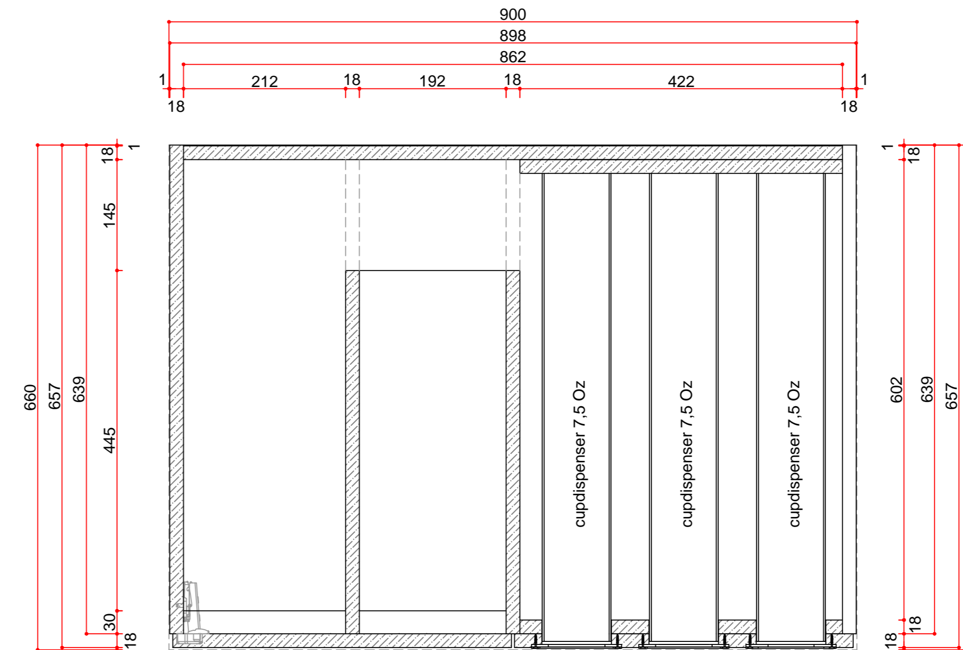
Horizontal section B-B
