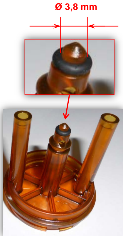
The pre-modification upper piston spare code is: 256750 It is no longer available
