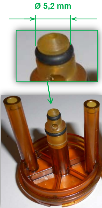
The new upper piston spare code is: 260204
