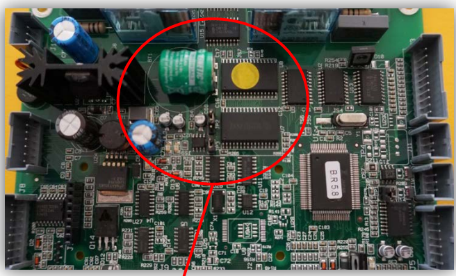
Pre-modification CPU - Actuator board 16 Bit 4M
